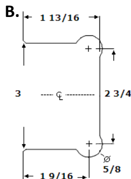
Hinge Cutout 'B' 3"W x 1.8125"D - Lobed/Mickey
