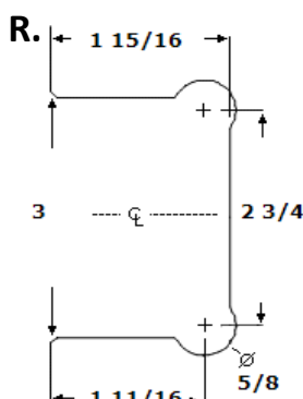
Hinge Cutout 'R' 3"W x 1.9375"D - Lobed/Mickey
