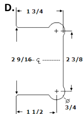
Hinge Cutout 'D' 2.5625"W x 1.75"D - Lobed/Mickey
