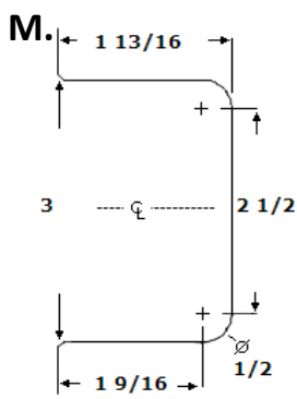
Hinge Cutout 'M' 3"W x 1.8125"D - Square
