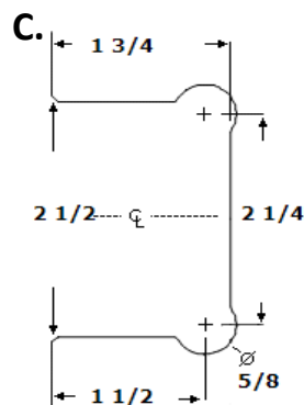
Hinge Cutout 'C' 2.5"W x 1.75"D - Lobed/Mickey
