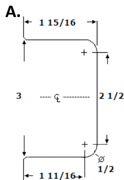
Hinge Cutout 'A' 3"W x 1.9375"D - Square
