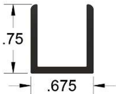
1/2 Deep U-Channel 144"
