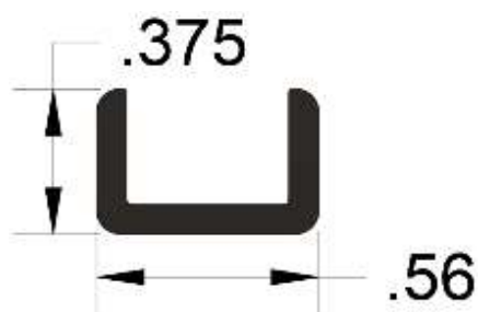
3/8 Shallow U-Channel 98"
