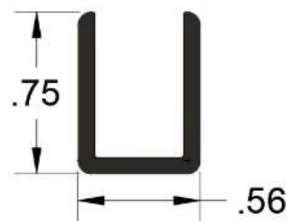
3/8 Deep U-Channel 144"
