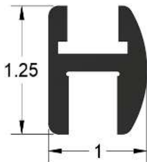
3/8" Euro Header
