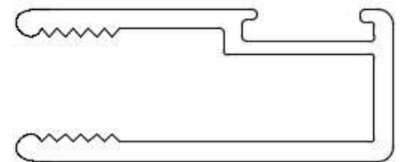
Magnetic Strike Stile E-MGSCH (E-553)
