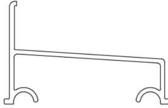
Framed Slider Bottom Track E-FBT (E-102)
