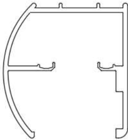
3/8" Semi-FL Slider Header E-HE38SFL (E-300)
