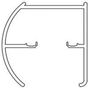
1/4" Semi-FL Slider Header E-HE14SFL (E-200)
