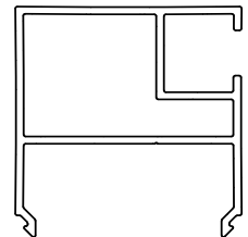
90 Deg. Slider Return Post E-90RP (E-114)
