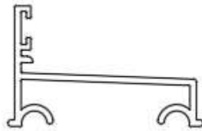
Semi-FL Slider Bottom Track E-BTSFL (E-202)
